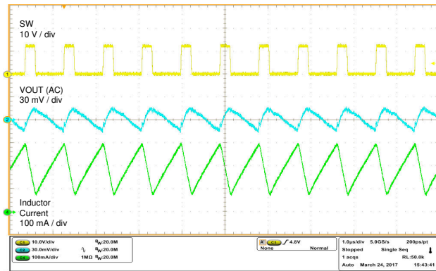
图 8-2. Switching Waveforms in PWM CCM Mode
