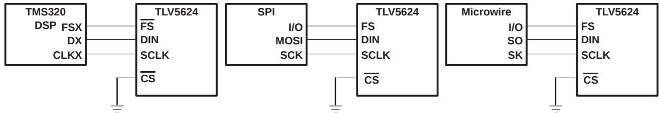
Figure 14. Three-Wire Interface
