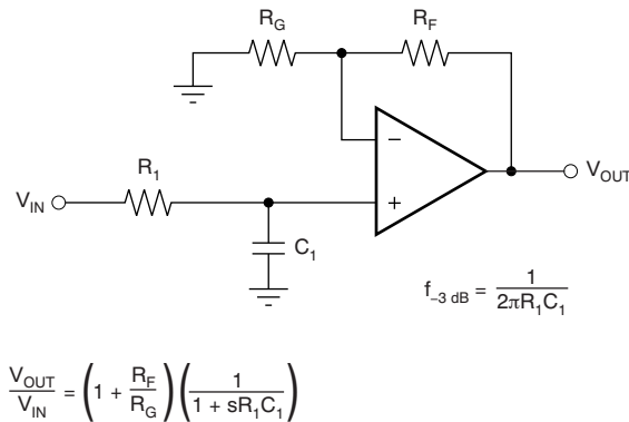
图 15. Single-Pole, Low-Pass Filter
