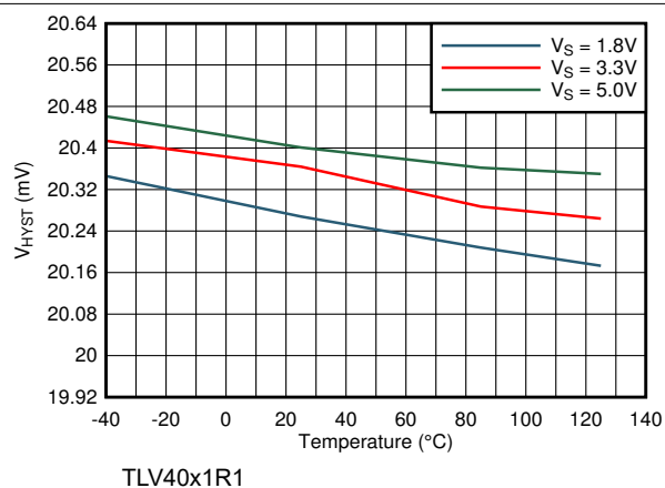
图 7-5. Hysteresis vs Temperature
