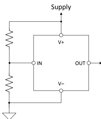
图 9-1. Supply Monitoring
