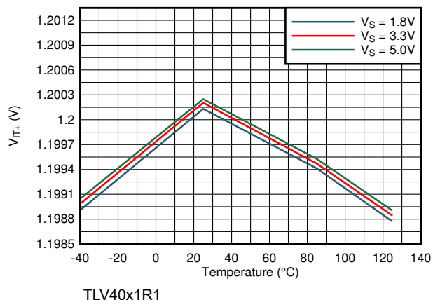
图 7-1. Positive Threshold vs Temperature
