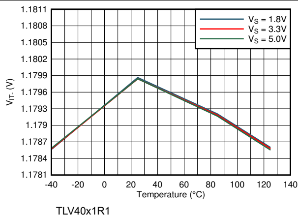
图 7-3. Negative Threshold vs Temperature
