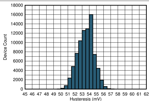
TLV4021S5x
