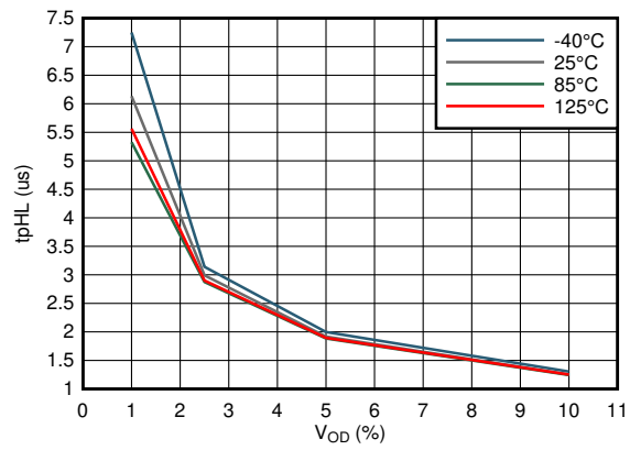
图 7-31. Propagation Delay High-Low vs Input Overdrive
