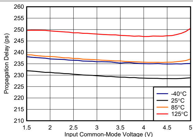
图 6-14. Propagation Delay vs. Common-Mode, 5 V
