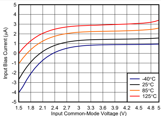
图 6-12. Bias Current vs. Common-Mode, 5 V
