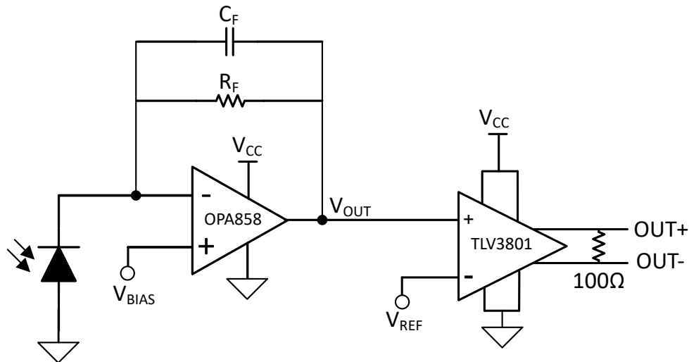
图 8-1. Optical Receiver
