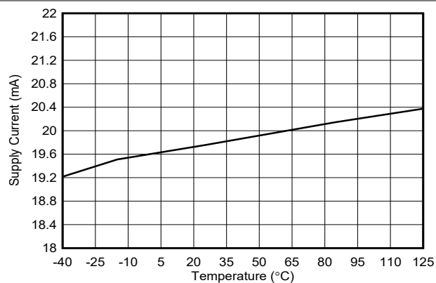
图 6-10. Supply Current vs. Temperature, Output High
