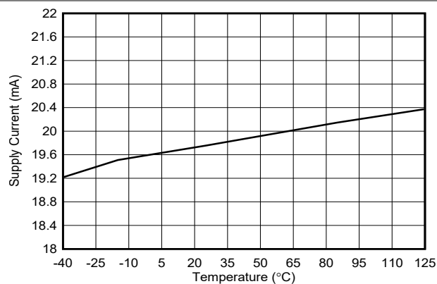
图 6-9. Supply Current vs. Temperature, Output Low
