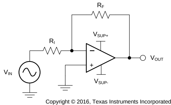
Figure 15. Application Schematic
