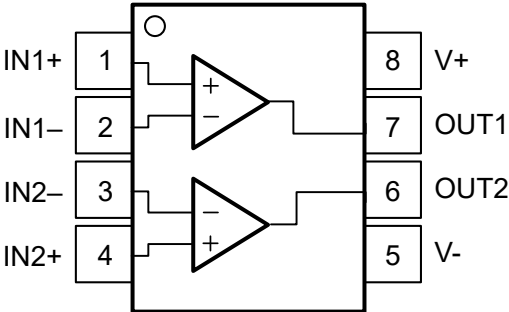
图 5-3. TLV3602 DGK, DSG Packages 8-Pin VSSOP, WSON
