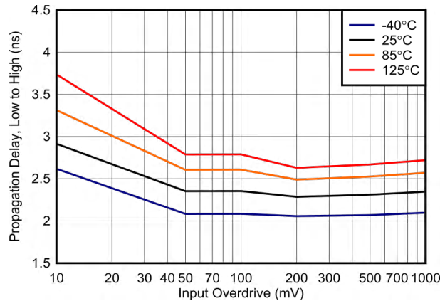
图 6-41. Propagation Delay, Low to High, 3.3 V
