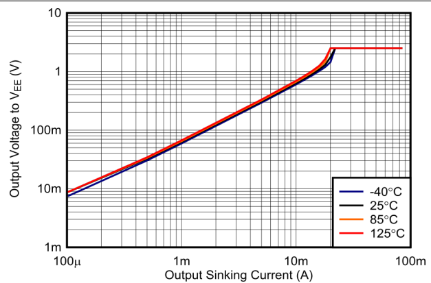
图 6-26. Output Voltage vs. Output Sinking Current, 2.5 V
