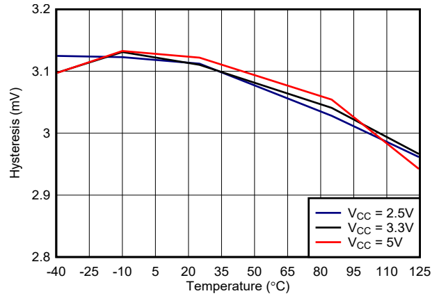
图 6-4. TLV3601 Hysteresis vs. Temperature
