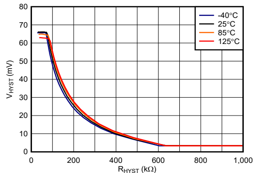
图 8-2. V_{\text{HYST}} (mV) vs R_{\text{HYST}} (kΩ), V_{\text{CC}} = 5\text{ V}
