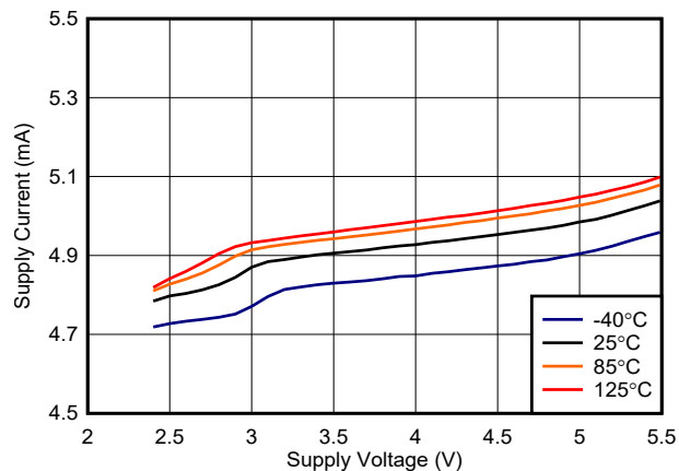
图 6-32. TLV3601 Supply Current vs. Voltage (Output High)
