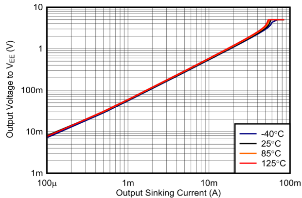
图 6-30. Output Voltage vs. Output Sinking Current, 5 V
