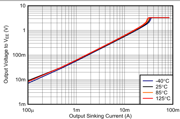
图 6-28. Output Voltage vs. Output Sinking Current, 3.3 V
