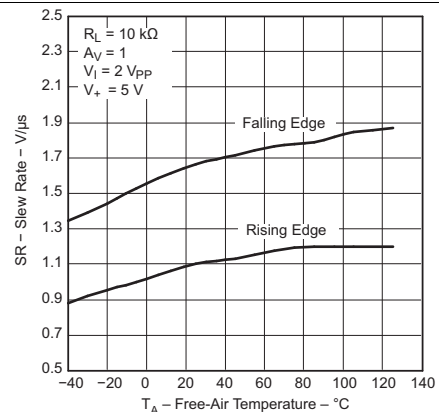
Figure 15. Slew Rate vs Temperature
