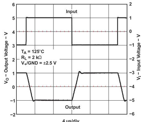
Figure 5-36. Large-Signal Inverting Response
