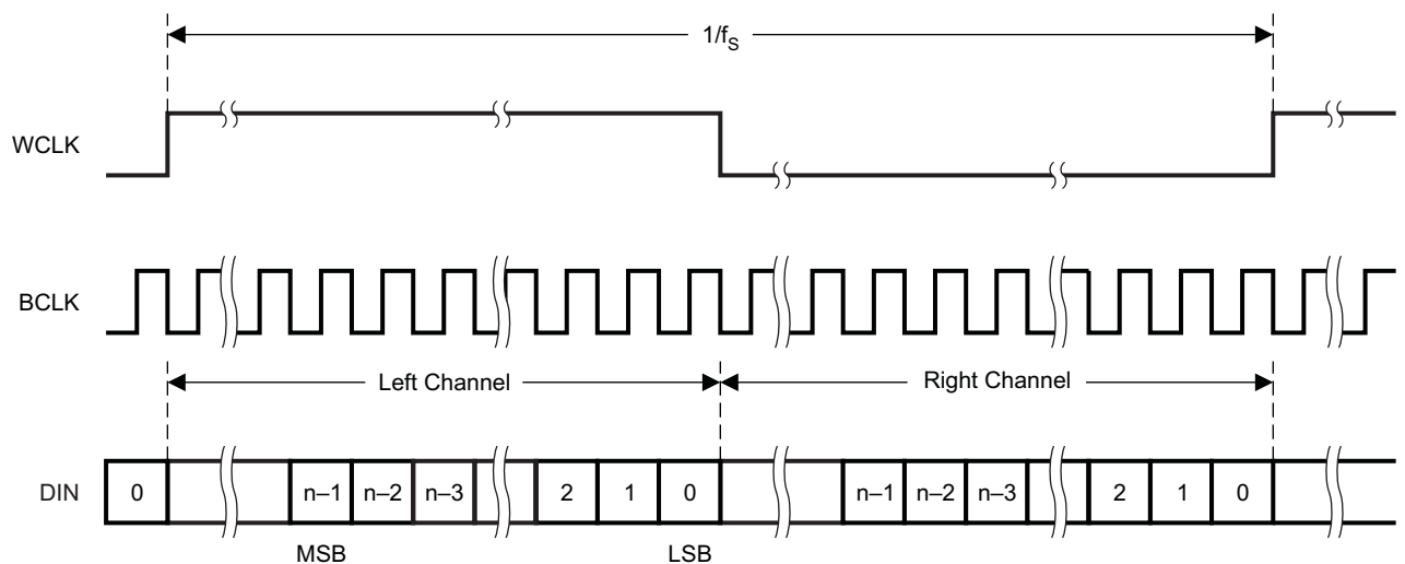
Figure 5-24. Timing Diagram for Right-Justified Mode
