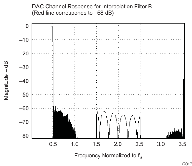
Figure 5-15. Frequency Response of Channel Interpolation Filter B
