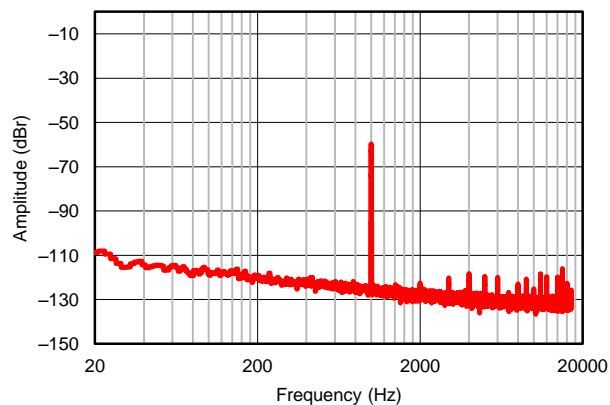
Figure 26. DAC Playback on Headphone Amplifier, Output Amplitude versus Frequency
