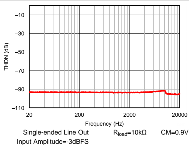
Figure 24. DAC Playback on Line Out Amplifier, Total Harmonic Distortion + Noise versus Input Frequency
