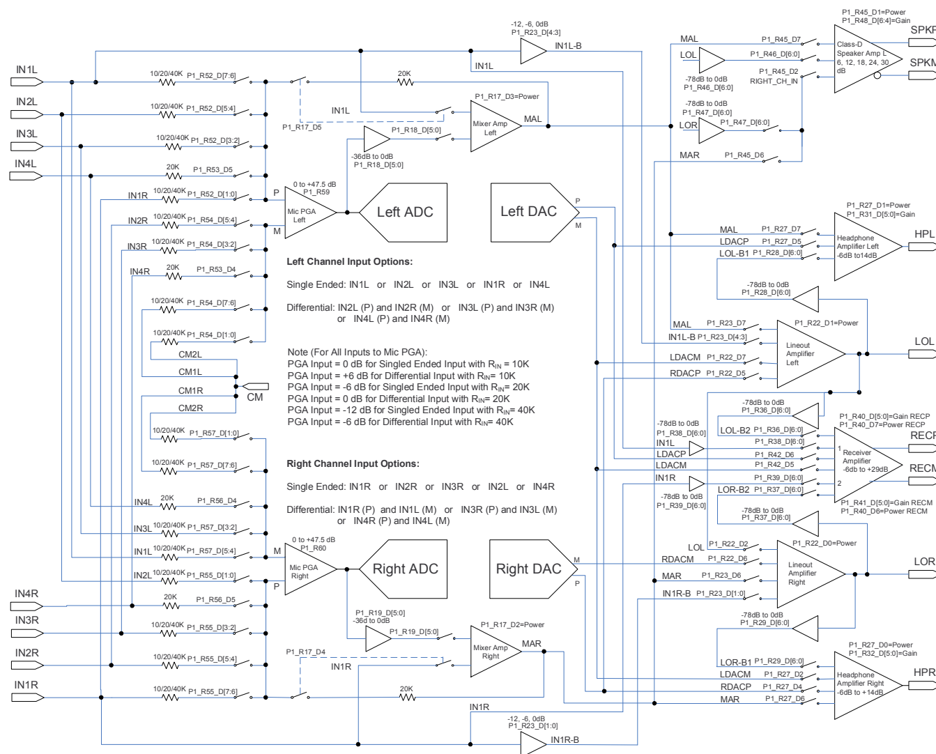
Figure 37. Analog Routing Diagram
