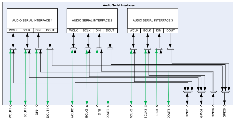
Figure 27. Typical Multiple Connections to Three Audio Serial Interfaces
