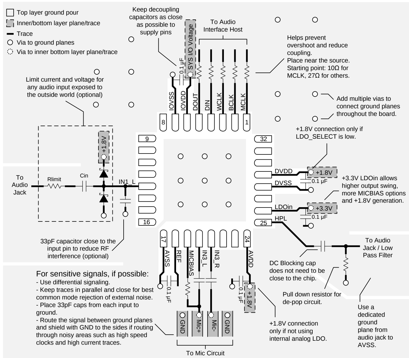
Figure 26. TLV320AIC3254 Layout
