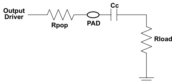
图 24. Conceptual Circuit for Pop-Free Power-up
