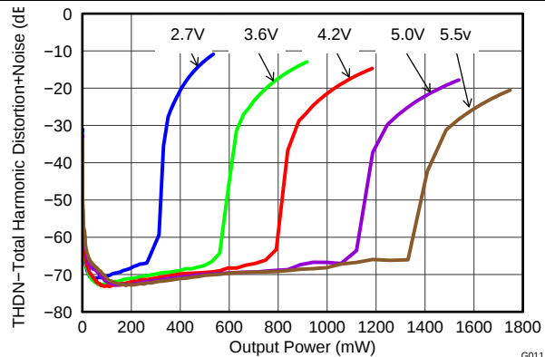
Figure 18. Total Harmonic Distortion + Noise vs Output Power with Different SLVDD/SRVDD/SPK_V Supplies, 8Ω Load, 12dB Gain
