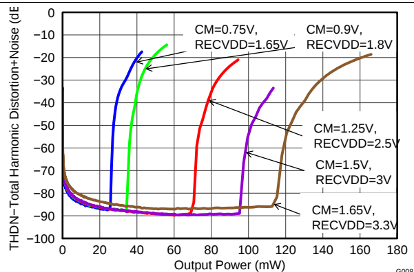
图 35. Total Harmonic Distortion+Noise vs Differential Receiver Output Power 32- \Omega Load
