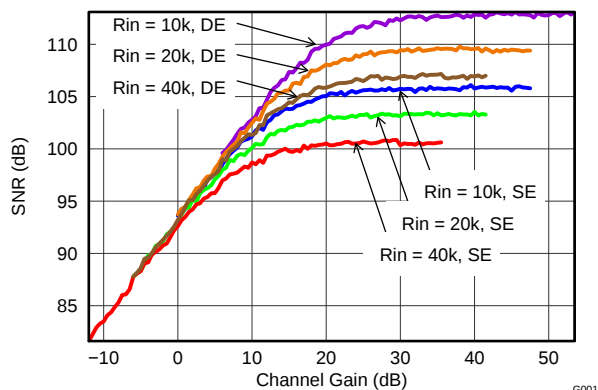
图 34. ADC SNR vs Channel Gain Input-Referred
