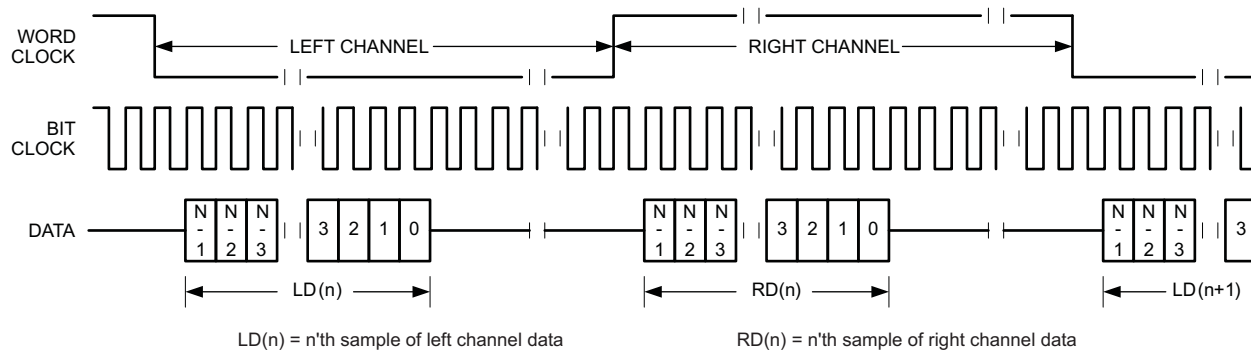
Figure 7-45. Timing Diagram for I²S Mode With Offset = 0 and Bit Clock Inverted
