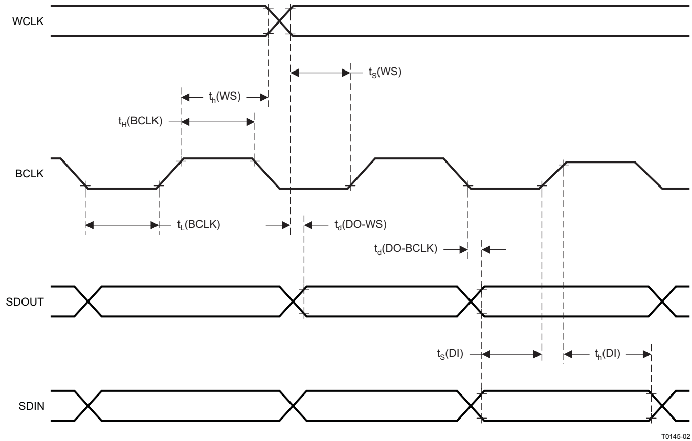
图 3. I²S, Left-Justified and Right-Justified Format Timing in Slave Mode
