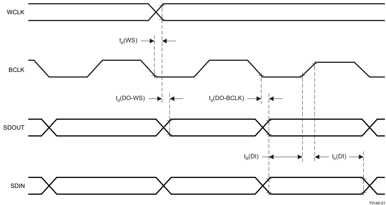
Figure 1. I²S/LJF/RJF Timing In Master Mode
