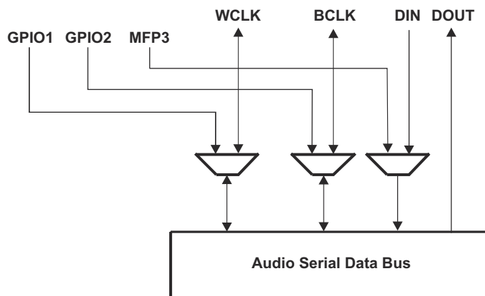
图 10-1. Alternate Audio Bus Multiplexing Function
