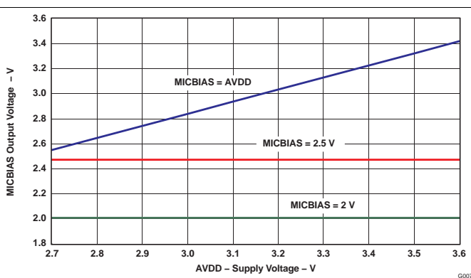
Figure 35. MICBIAS Output Voltage vs AVDD
