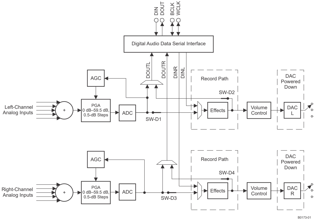
图 7-11. Record-Only Mode With Digital Processing Path Enabled
