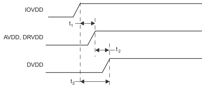
图 9-6. Power-Supply Sequencing
