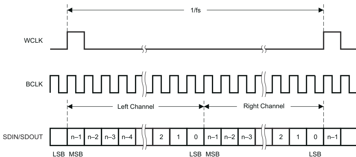
图 7-19. DSP Serial Data Bus Mode Operation
