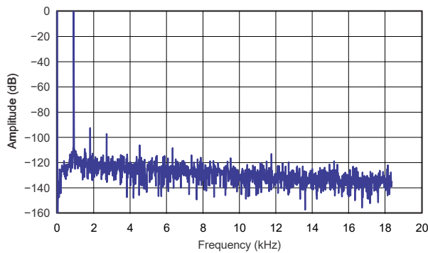
图 9-2. DAC to Line Output FFT at 1-kHz Signal Plot
