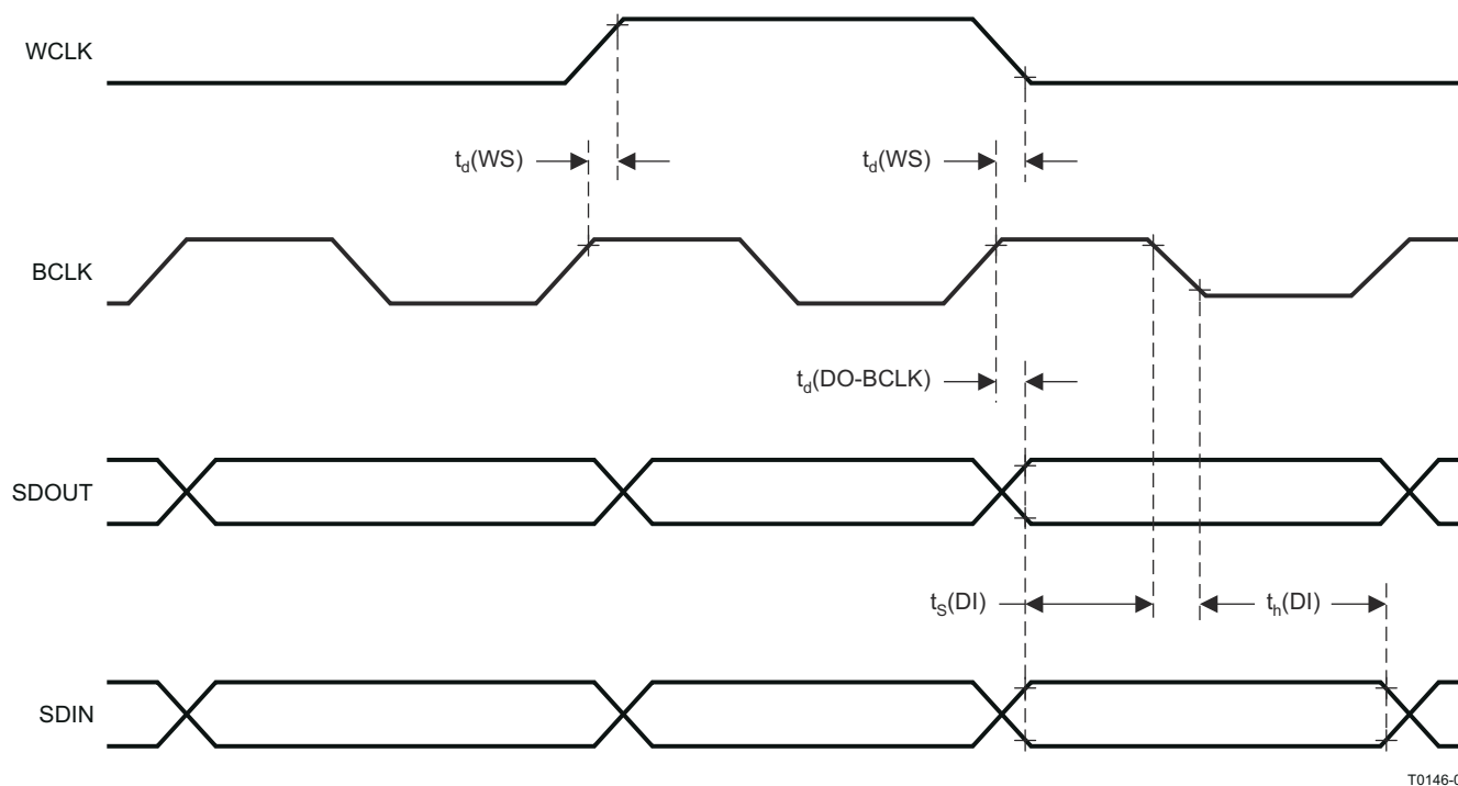
图 6-3. DSP Timing in Master Mode
