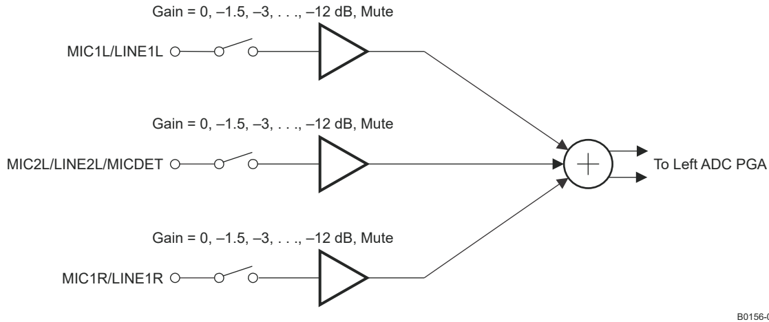
图 7-4. Single-Ended Analog Input Mixing Configuration
