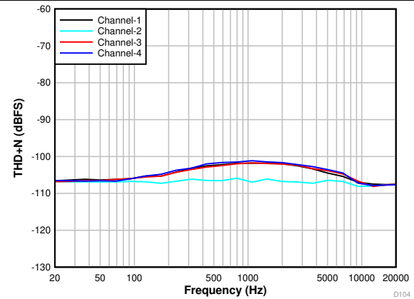
图 12. THD+N vs Input Frequency With a -1-dBr Input
