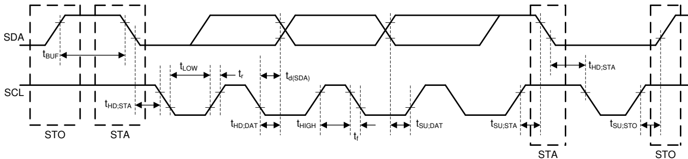
图 1. I²C Interface Timing Diagram
