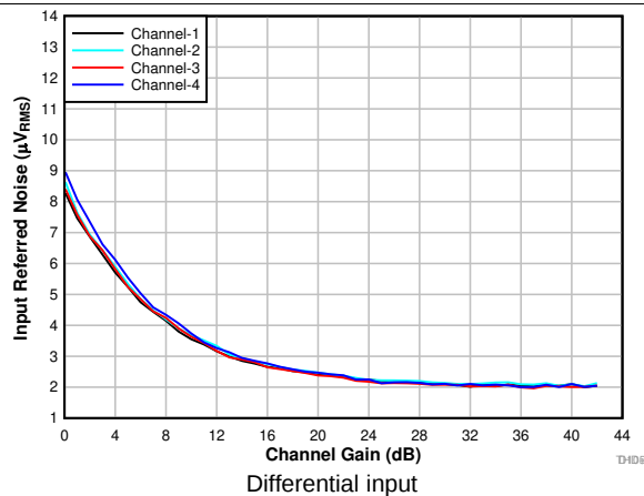
图 13. Input-Referred Noise vs Channel Gain Differential input
