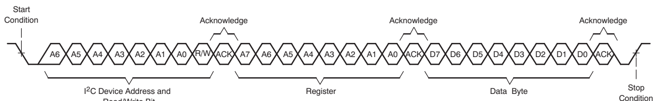
图 89. I 2 C Single-Byte Write Transfer
