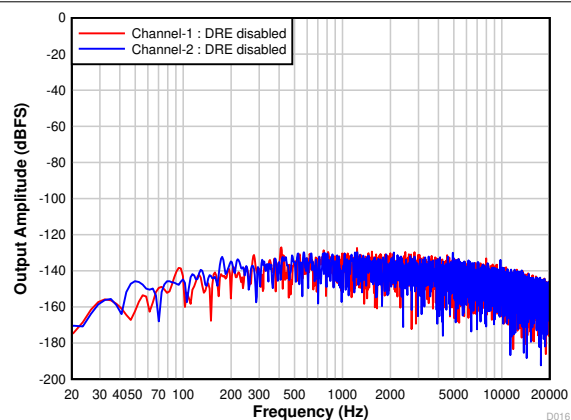
图 7-19. FFT With Idle Input With DRE Disabled
