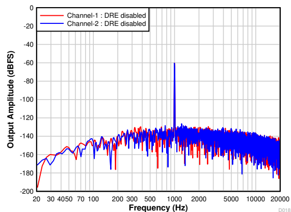
图 7-21. FFT With a -60-dBr Input With DRE Disabled
