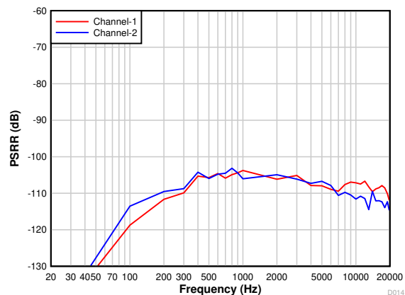
图 7-17. Power-Supply Rejection Ratio vs Ripple Frequency With 100-mV pp Amplitude
