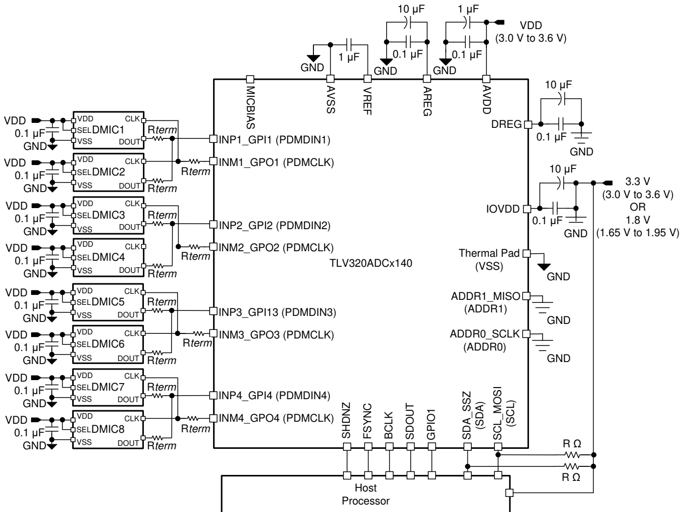
图 168. Eight-Channel Digital PDM Microphone Recording Diagram
