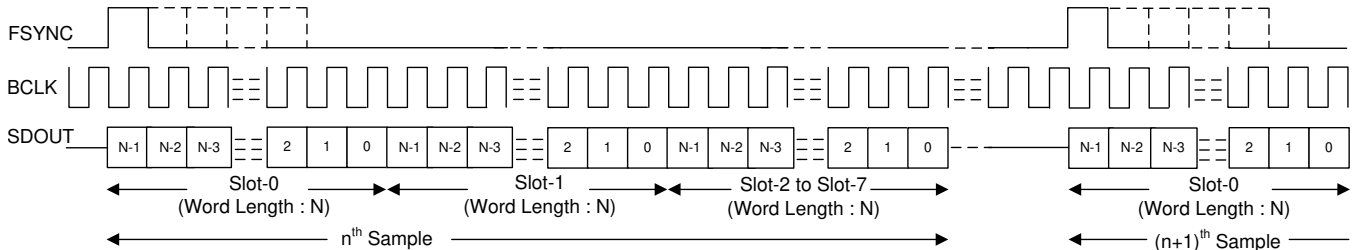
图 20. TDM Mode Protocol Timing (TX_OFFSET = 0 and BCLK_POL = 1)
