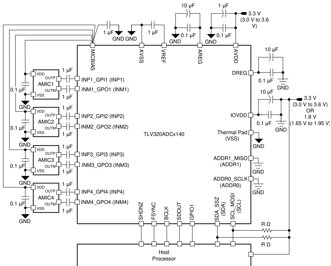
图 165. Four-Channel Analog Microphone Recording Diagram
