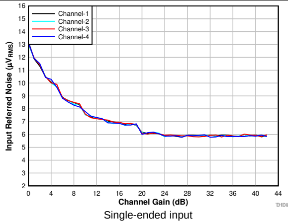
图 11. Input-Referred Noise vs Channel Gain
