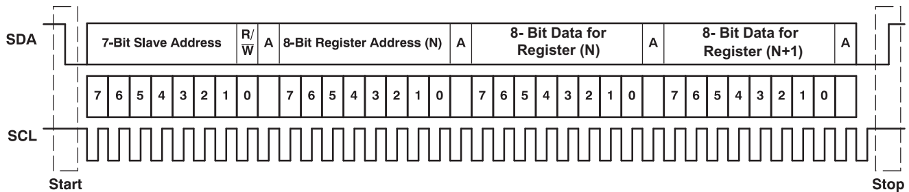
图 82. Typical I²C Sequence
