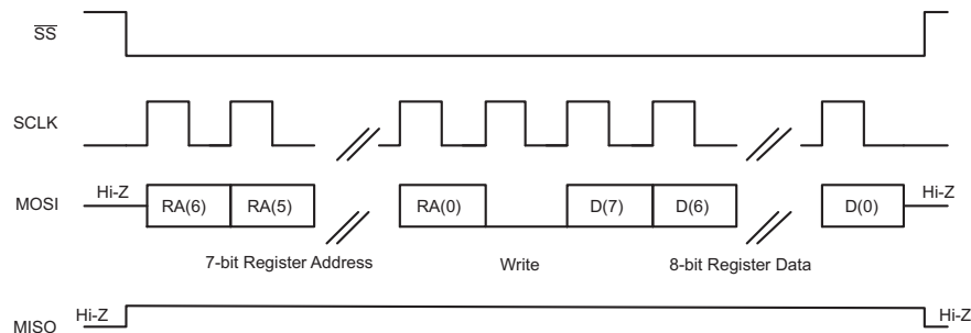
图 87. SPI Single-Byte Write Transfer
