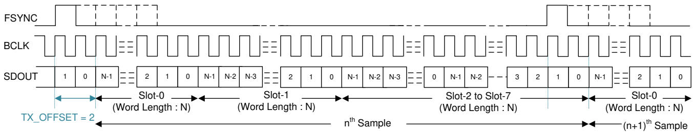
图 19. TDM Mode Protocol Timing (No Idle BCLK Cycles, TX_OFFSET = 2)
