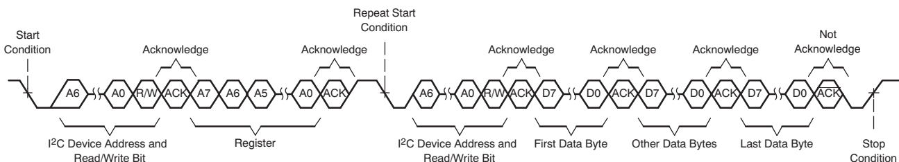
图 86. I 2 C Multiple-Byte Read Transfer
