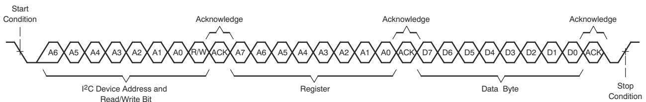
图 8-67. I²C Single-Byte Write Transfer
