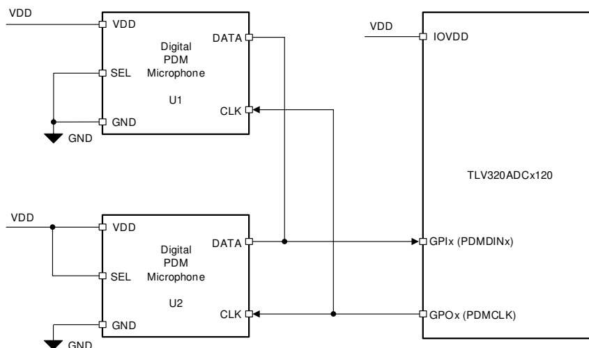
图 8-64. Digital PDM Microphones Connection Diagram for the TLV320ADC3120
