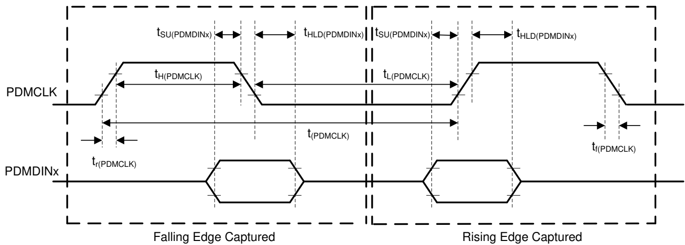
图 7-3. PDM Digital Microphone Interface Timing Diagram
