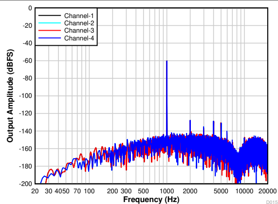
图 7-18. PDM Input FFT With a -60-dBr Input
