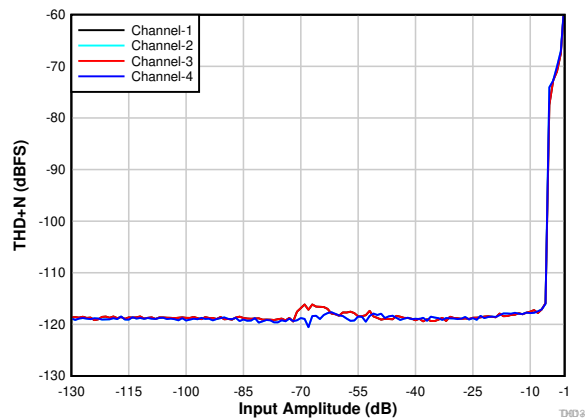
图 7-16. PDM Input THD+N vs Input Amplitude
