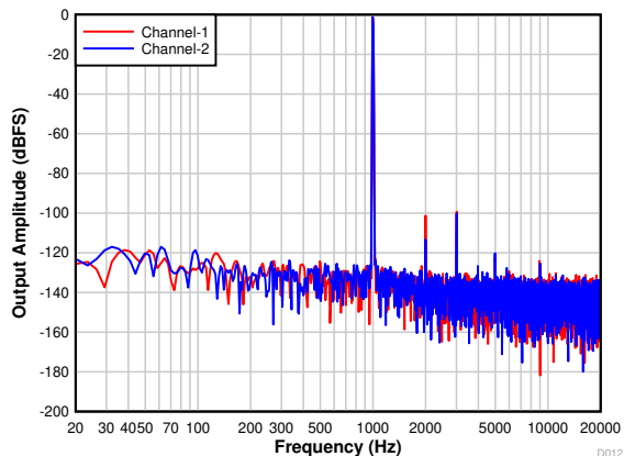
图 7-15. FFT With a -1-dBr Input
