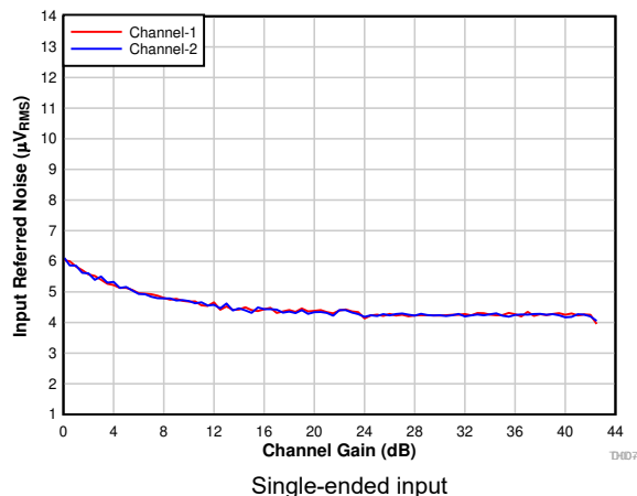
图 7-10. Input-Referred Noise vs Channel Gain
