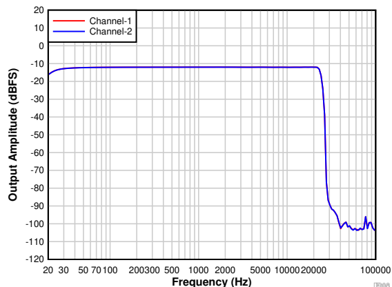
图 7-11. Frequency Response With a -12-dBr Input
