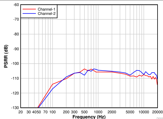
图 7-12. Power-Supply Rejection Ratio vs Ripple Frequency With 100-mV pp Amplitude
