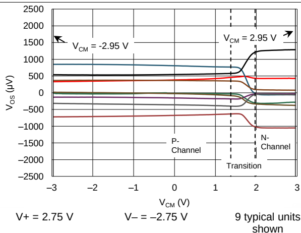
图 2. Offset Voltage vs Common-Mode Voltage
