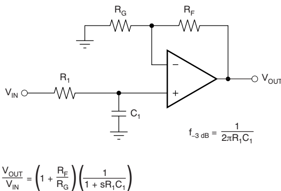
Figure 17. Single-Pole, Low-Pass Filter
