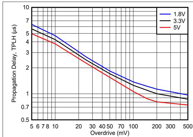
图 6-30. Low to High Propagation Delay vs. Overdrive
