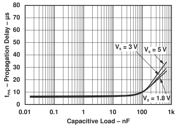
图 6-5. PROPAGATION DELAY ( t_{PHL} ) vs CAPACITIVE LOAD
