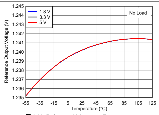
图 6-33. Reference Voltage vs. Temperature
