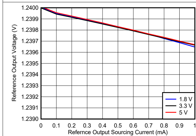
图 6-34. Reference Voltage vs. Reference Output Sourcing Current
