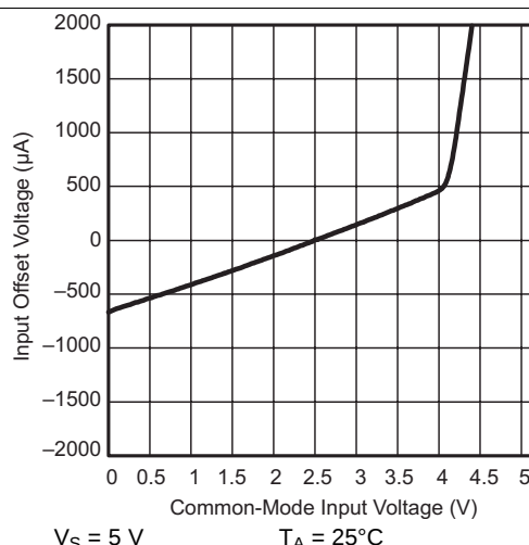
Figure 2. Input Offset Voltage vs Common-Mode Input Voltage
