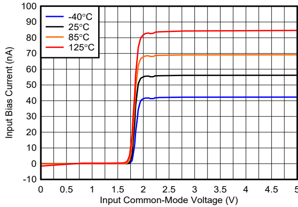
图 6-9. Bias Current vs. Common-Mode, 1.8 V
