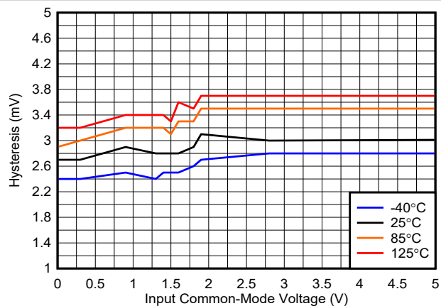
图 6-4. Hysteresis vs. Common-Mode, 1.8 V
