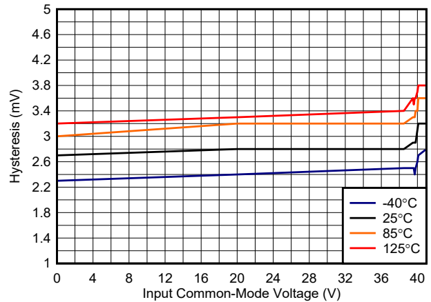
图 6-8. Hysteresis vs. Common-Mode, 40 V
