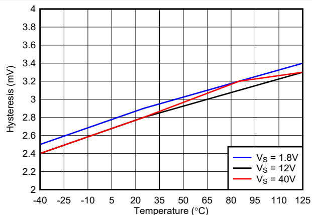
图 6-2. Hysteresis vs. Temperature
