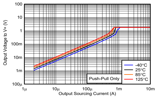
图 6-13. Output Voltage vs. Output Sourcing Current, 1.8V
