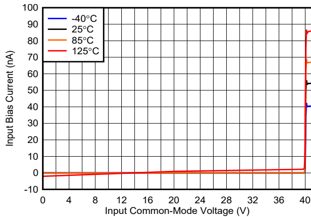
图 6-11. Bias Current vs. Common-Mode, 40 V
