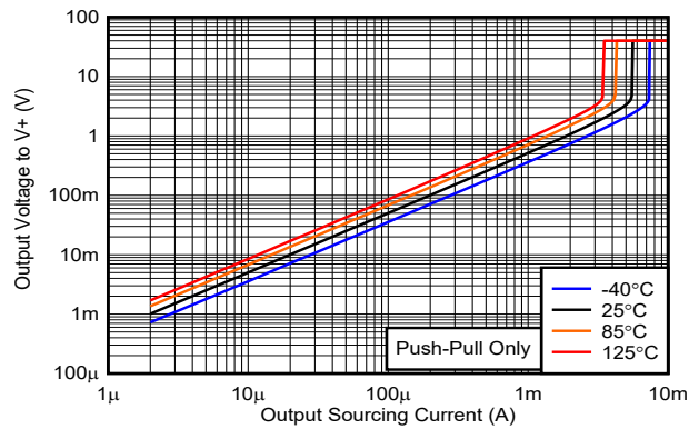
图 6-17. Output Voltage vs. Output Sourcing Current, 40V
