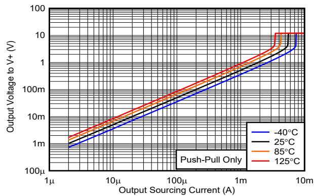
图 6-15. Output Voltage vs. Output Sourcing Current, 12V
