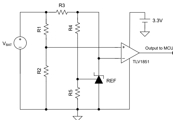
图 7-9. Undervoltage Detection
