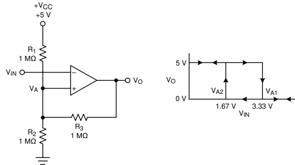
图 7-3. TLV185x in an Inverting Configuration With Hysteresis
