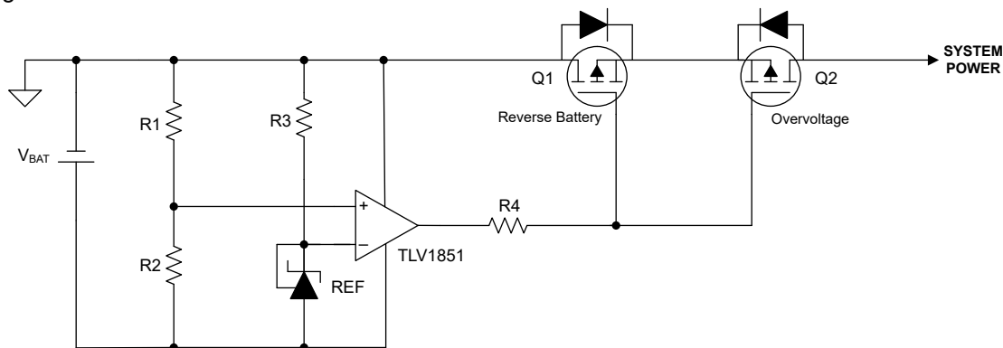
图 7-10. Reverse Battery and Overvoltage Protection Scheme
