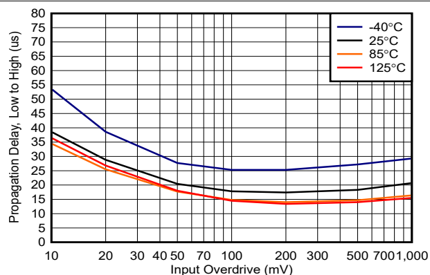
图 5-28. Propagation Delay, Low to High, 1.8V, Push-Pull
