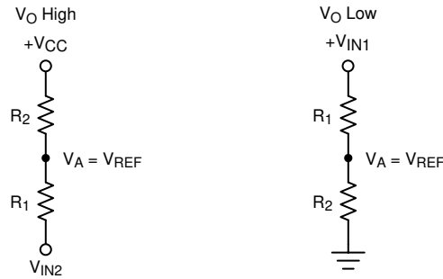
图 7-6. Non-Inverting Configuration Resistor Networks
