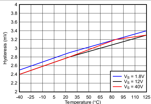
图 5-2. Hysteresis vs. Temperature
