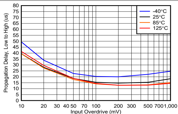
图 5-30. Propagation Delay, Low to High, 12V, Push-Pull
