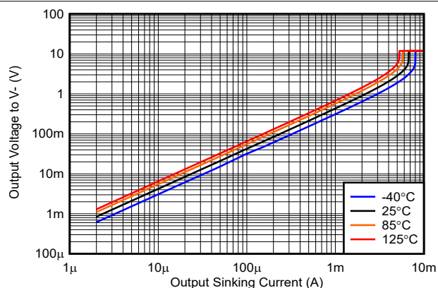
图 5-16. Output Voltage vs. Output Sinking Current, 12V
