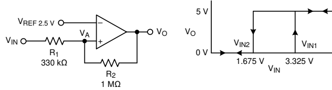
图 7-5. TLV185x in a Non-Inverting Configuration With Hysteresis
