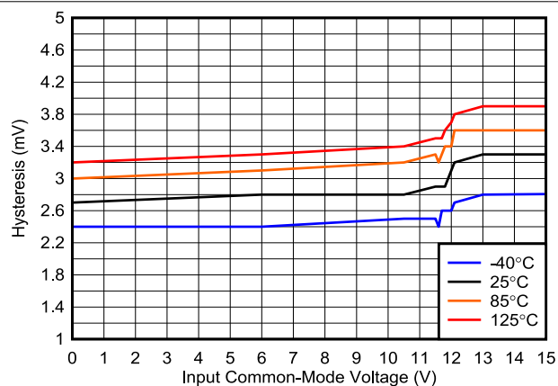
图 5-6. Hysteresis vs. Common-Mode, 12V
