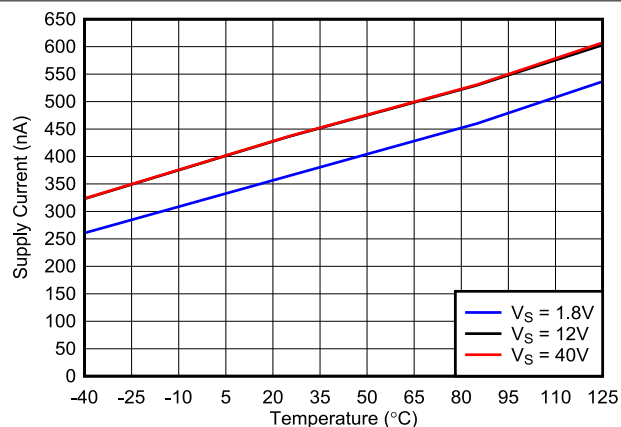
图 5-26. Supply Current vs. Temperature (Output High), Open Drain
