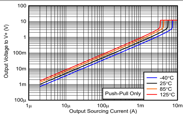
图 5-15. Output Voltage vs. Output Sourcing Current, 12V
