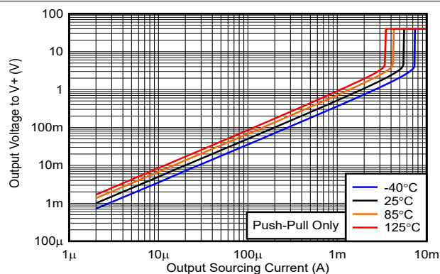
图 5-17. Output Voltage vs. Output Sourcing Current, 40V
