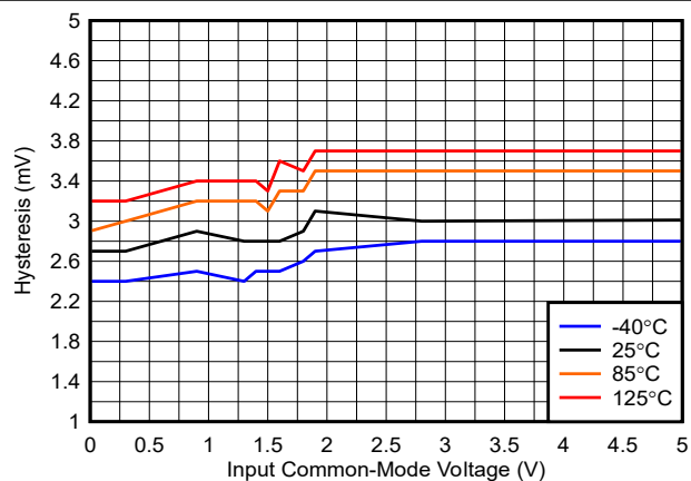
图 5-4. Hysteresis vs. Common-Mode, 1.8V
