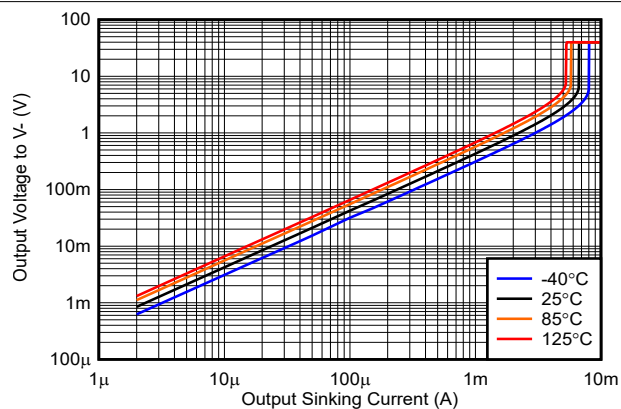
图 5-18. Output Voltage vs. Output Sinking Current, 40V
