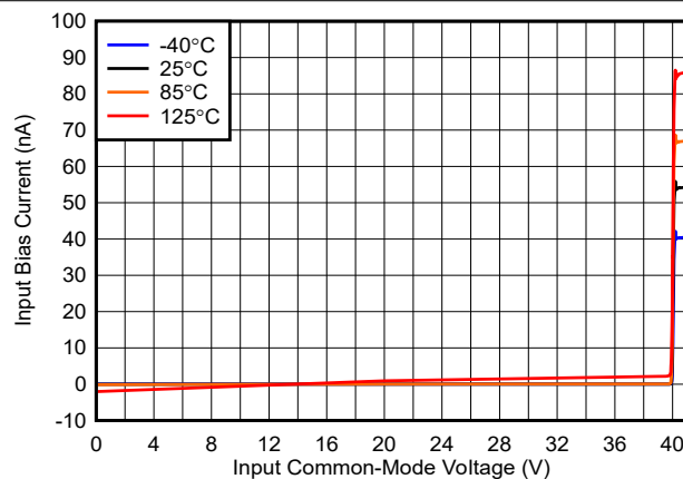
图 5-11. Bias Current vs. Common-Mode, 40V
