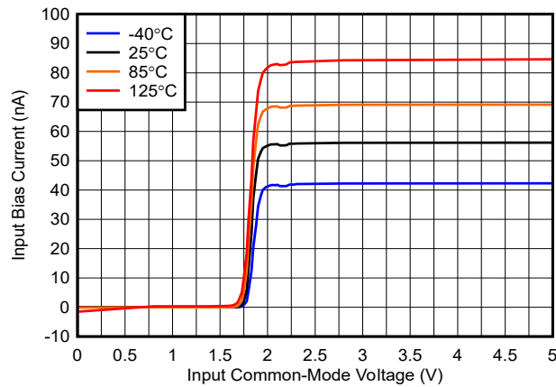
图 5-9. Bias Current vs. Common-Mode, 1.8V
