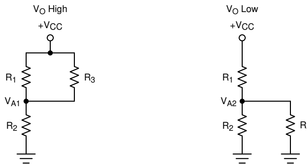
图 7-4. Inverting Configuration Resistor Equivalent Networks
