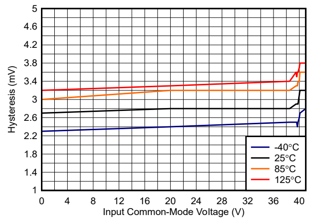
图 5-8. Hysteresis vs. Common-Mode, 40V
