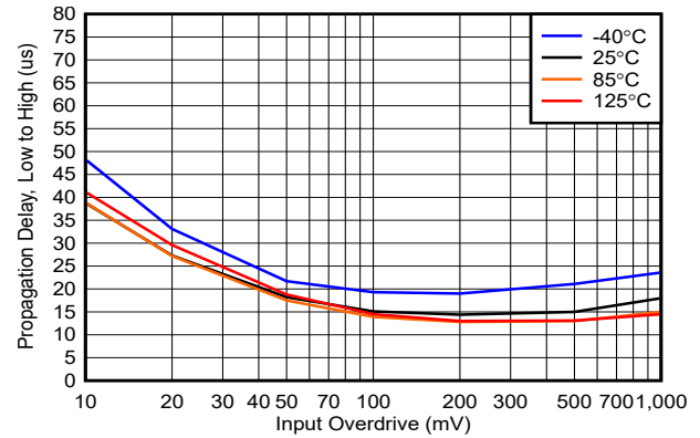
图 5-32. Propagation Delay, Low to High, 40V, Push-Pull
