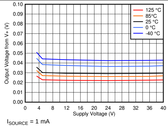
图 24. Output High Voltage vs. Supply Voltage
