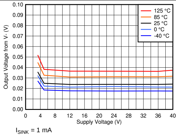
图 23. Output Low Voltage vs. Supply Voltage
