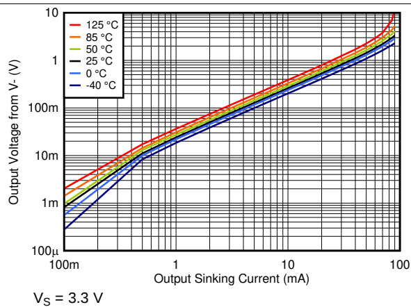
图 25. Output Voltage vs. Output Sinking Current at 3.3V
