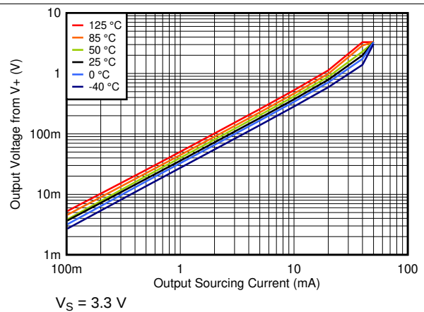
图 26. Output Voltage vs. Output Sourcing Current at 3.3V
