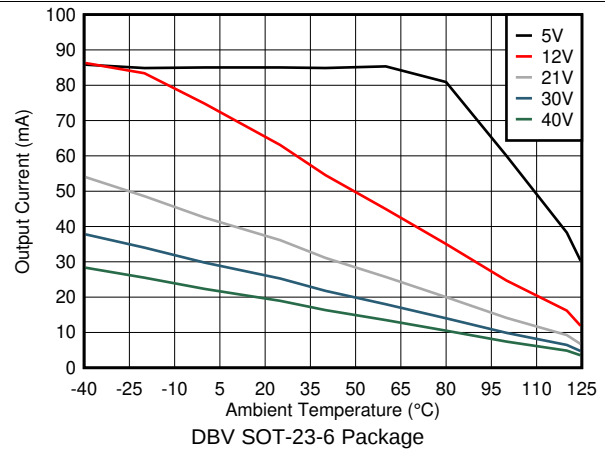
图 22. Maximum Continuous Output Current vs. Ambient Temperature
