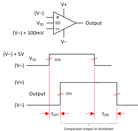
图 2. Shutdown Timing
