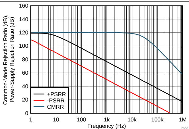
图 6. CMRR and PSRR vs Frequency (Referred-to-Input)
