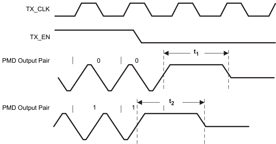
Figure 9-14. 10Base-T Transmit Timing (End of Packet)
