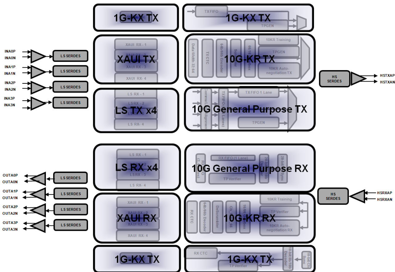
Figure 2-2. A Simplified One Channel Block Diagram of the TLK10232 Data Paths
