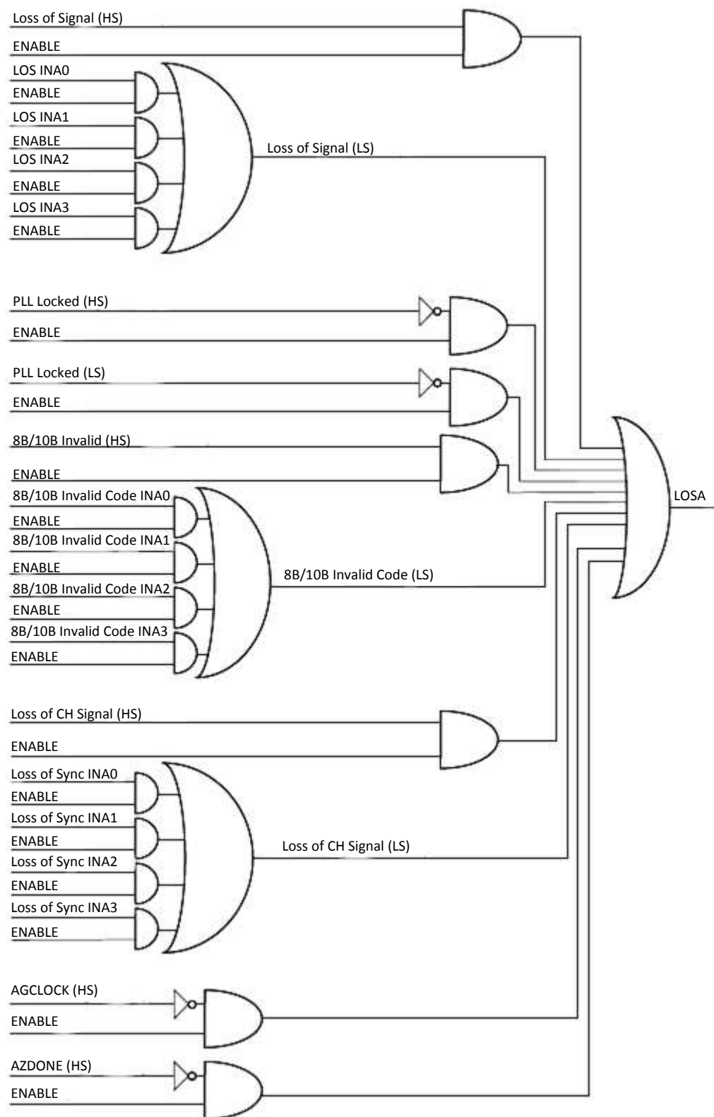
Figure 7-18. LOSA – Logic Circuit Implementation
