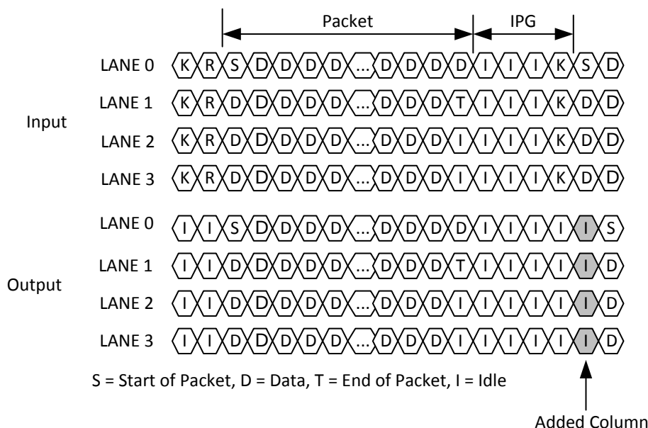
Figure 7-4. Clock Tolerance Compensation: Add
