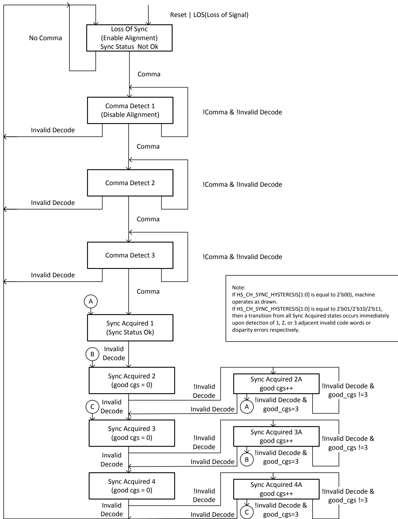
Figure 7-3. Channel Synchronization Flowchart
