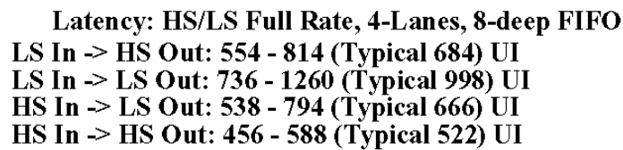
Figure 3-5. TLK10022 Transmit / Receive Latency
