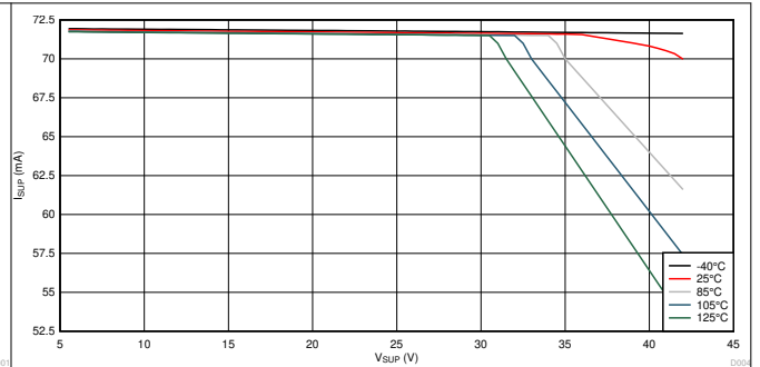
V_{CC} = 5\text{ V} I_{CC}\text{ Load} = 70\text{ mA} Normal Mode 图 7-2. I_{SUP} vs V_{SUP} Across Temperature
