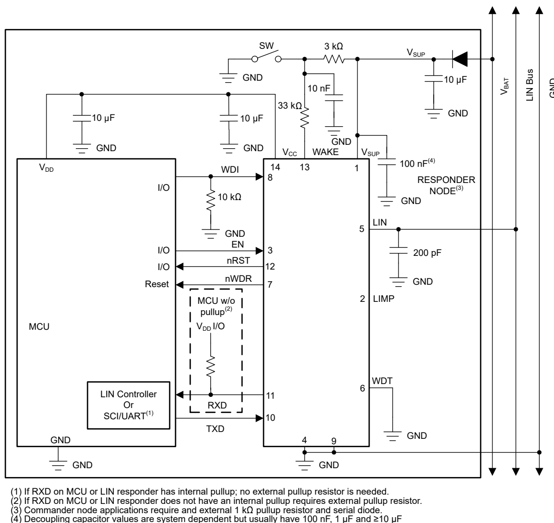
图 10-1. Typical LIN Controller in Pin Control Mode
