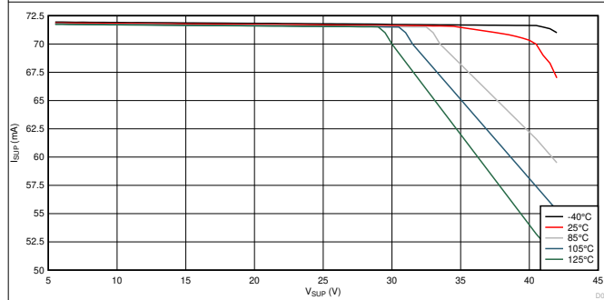
V_{CC} = 3.3\text{ V} I_{CC}\text{ Load} = 70\text{ mA} Normal Mode 图 7-3. I_{SUP} vs V_{SUP} Across Temperature
