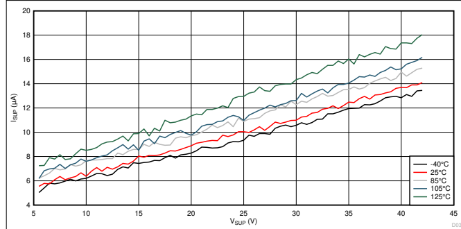
V_{CC} = 3.3\text{ V} Sleep Mode 图 7-5. I_{SUP} vs V_{SUP} Across Temperature
