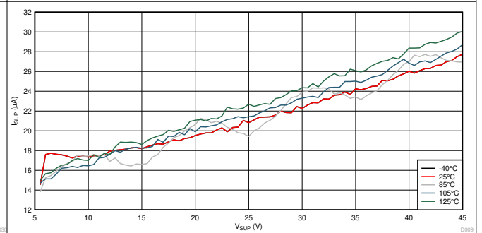
V_{CC} = 5\text{ V} Sleep Mode 图 7-4. I_{SUP} vs V_{SUP} Across Temperature
