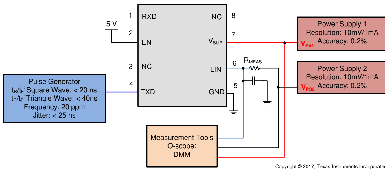
图 8-11. Test Circuit Slope Control and Duty Cycle Param 27, 28, 29, 30
