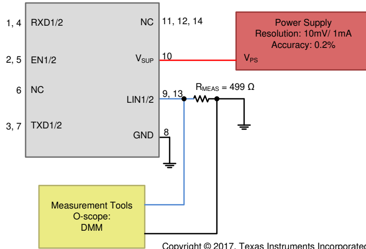
图 8-6. Test Circuit for I_{BUS\_PAS\_dom} ; TXD = Recessive State V_{BUS} = 0 V, Parameters 13
