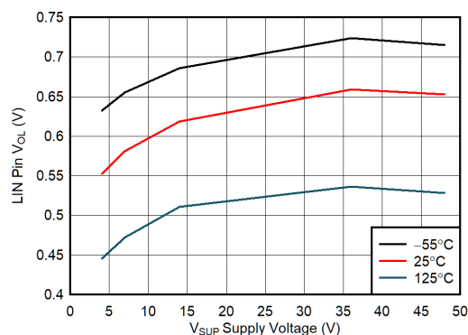
图 7-2. V_{OL} vs V_{SUP} and Temperature
