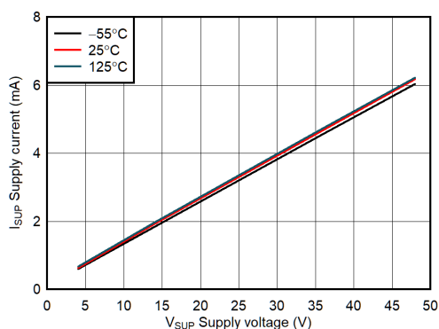
图 7-3. Supply Current vs Voltage Supply Across Temperature
