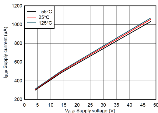
图 7-4. Supply Current vs Voltage Supply Across Temperature
