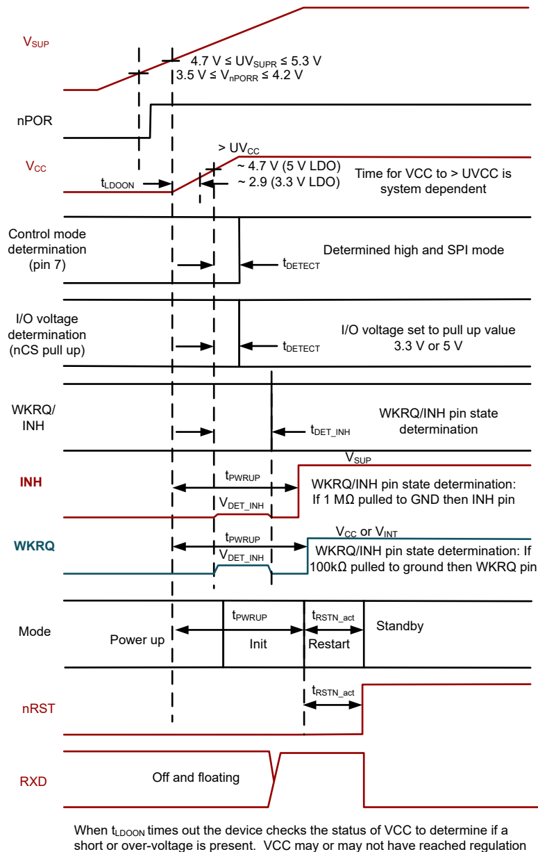
图 8-6. Power up timing diagram for pin 7 pulled high up
