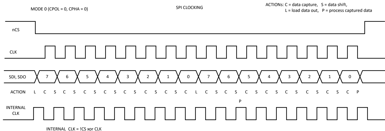
图 8-54. SPI Clocking
