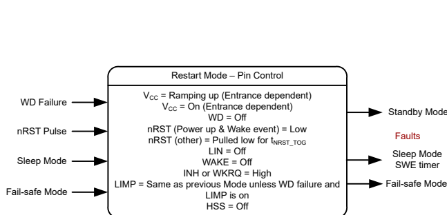
图 8-38. Restart Mode Pin Control
