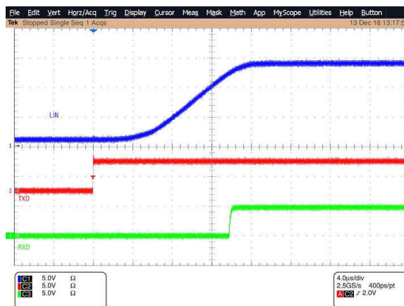
图 9-13. Dominant to Recessive Propagation Delay
