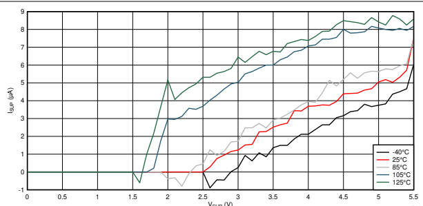
图 9-8. I_{SUP} vs V_{SUP} Across Temperature
