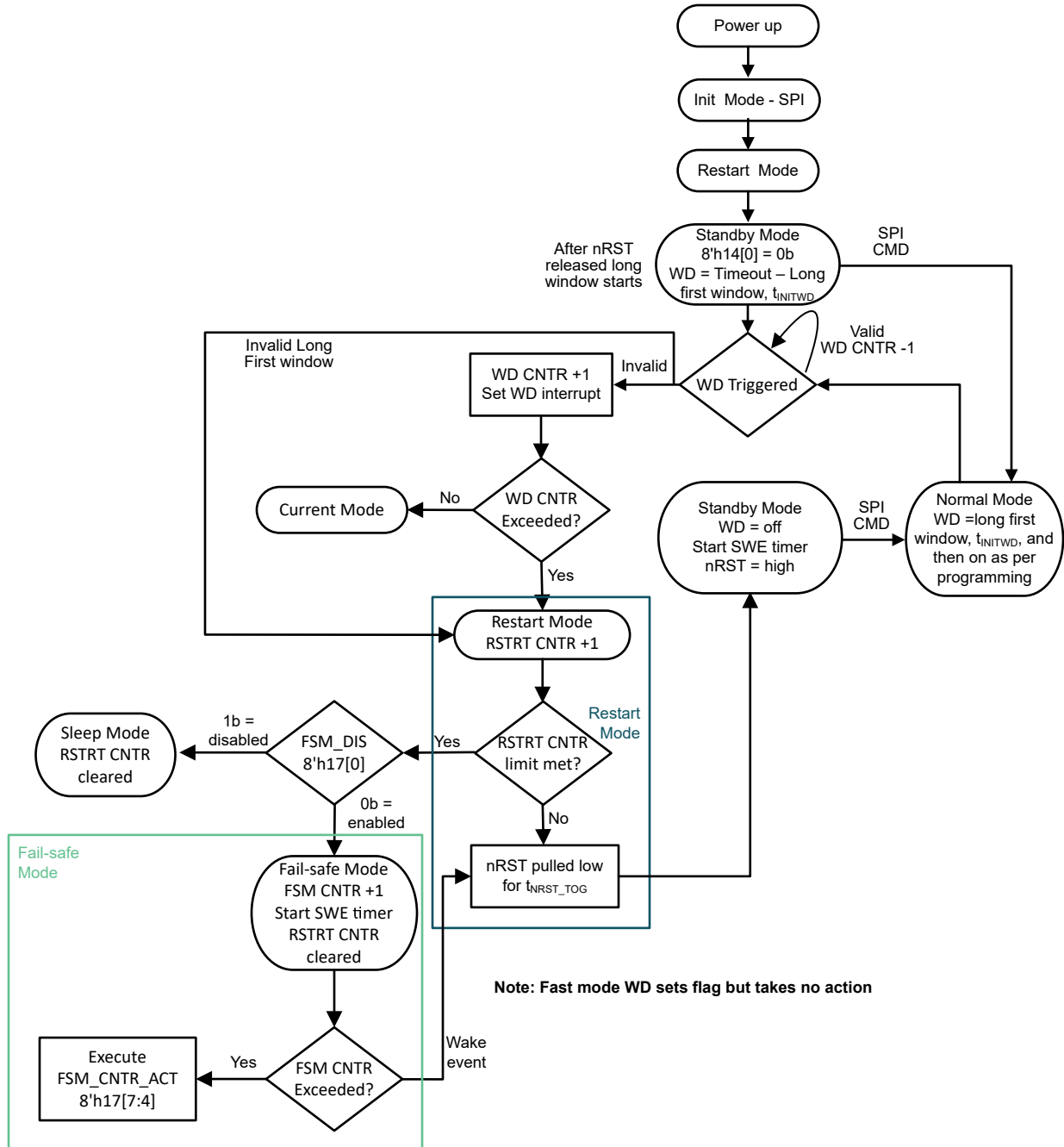
图 8-18. Watchdog state diagram in SPI mode; Standby Mode Disabled
