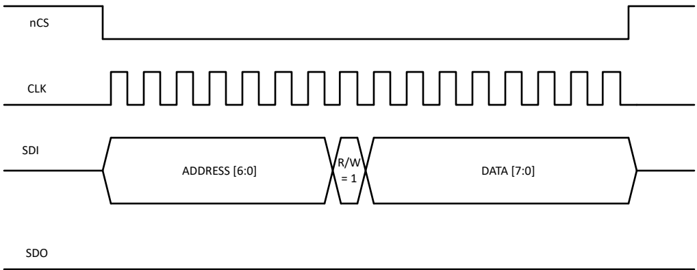
图 8-50. SPI Write
