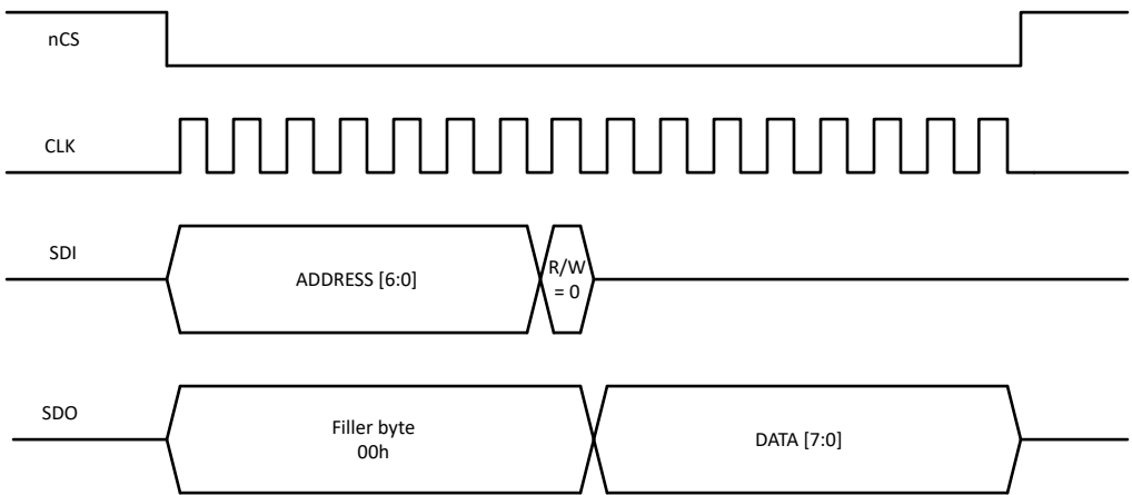
图 8-51. SPI Read
