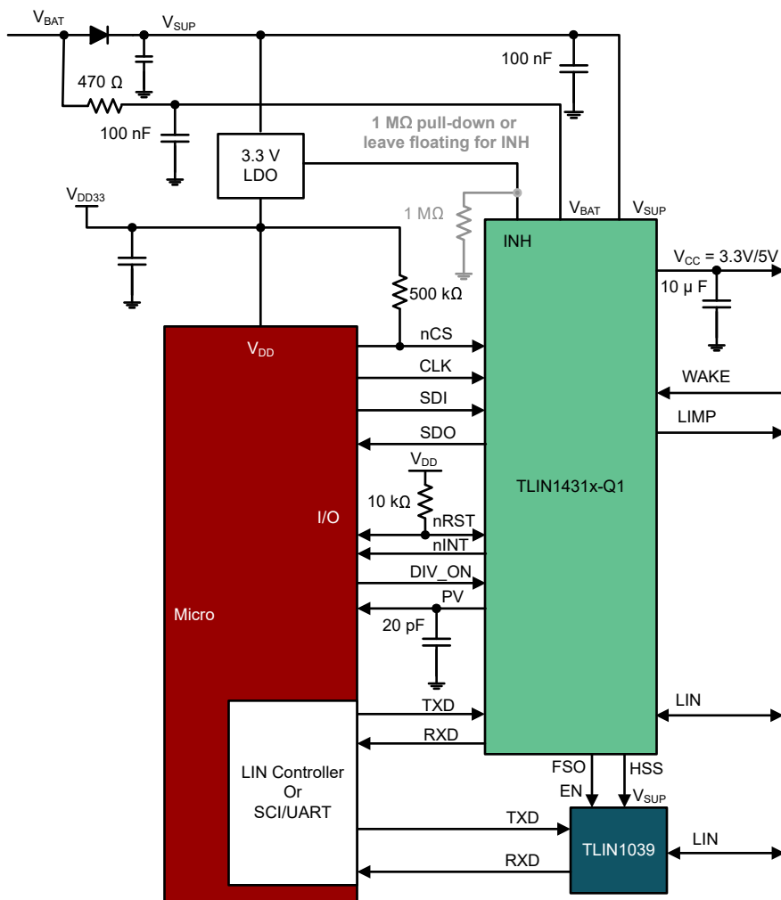
图 8-19. Channel Expansion: LIN Transceiver
