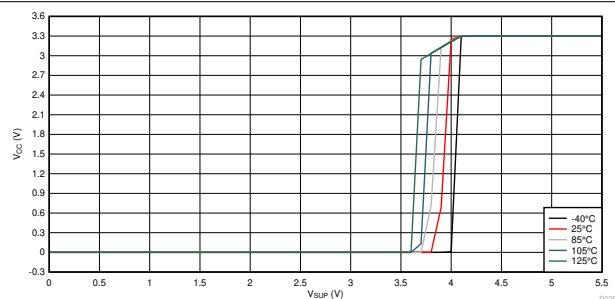
图 9-5. V_{CC} vs V_{SUP} Across Temperature
