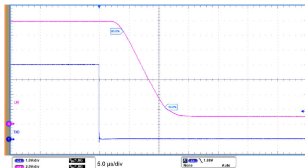
图 10-2. Recessive to Dominant Propagation
