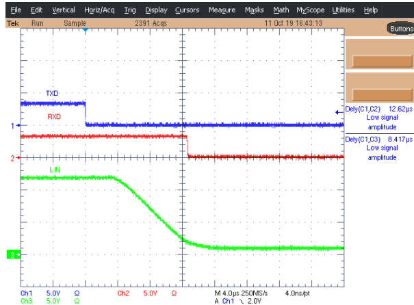
图 10-8. Recessive to Dominant Propagation Delay
