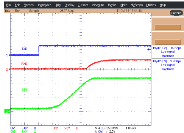
图 10-7. Dominant to Recessive Propagation Delay
