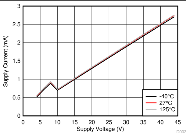
图 6-3. Dominant I_{SUP} vs V_{SUP} and Temperature
