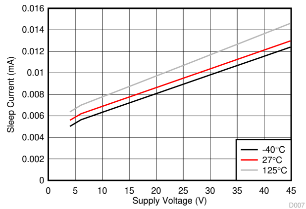
图 6-7. Sleep Current vs V_{SUP} and Temperature
