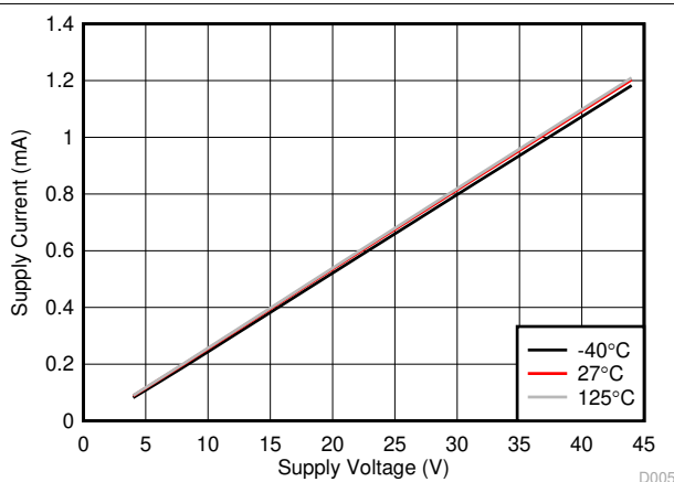
图 6-5. Standby Dominant I_{SUP} vs V_{SUP} and Temperature
