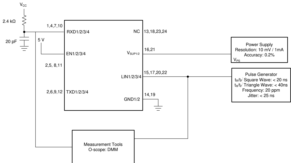
图 7-13. Propagation Delay Test Circuit
