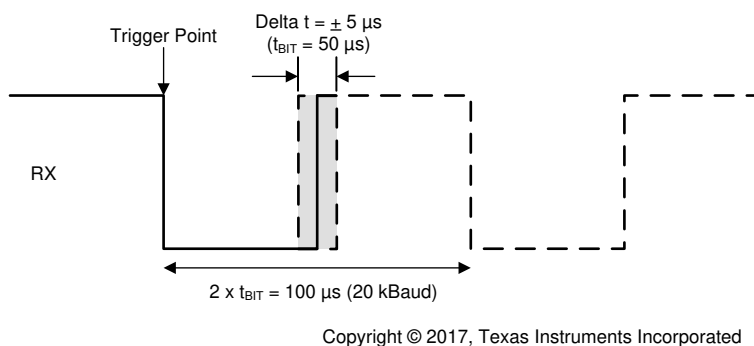
图 8-2. RX Response: Operating Voltage Range
