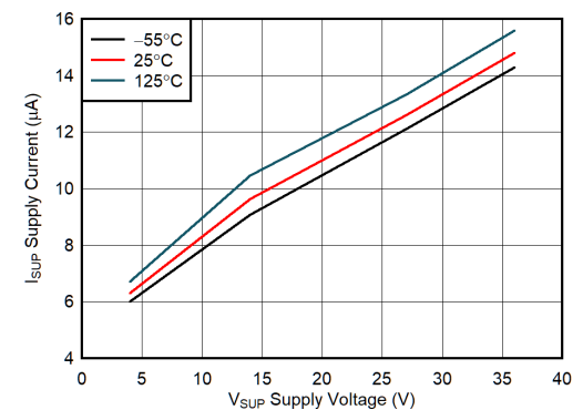
图 7-6. Supply Current vs Voltage Supply and Temperature
