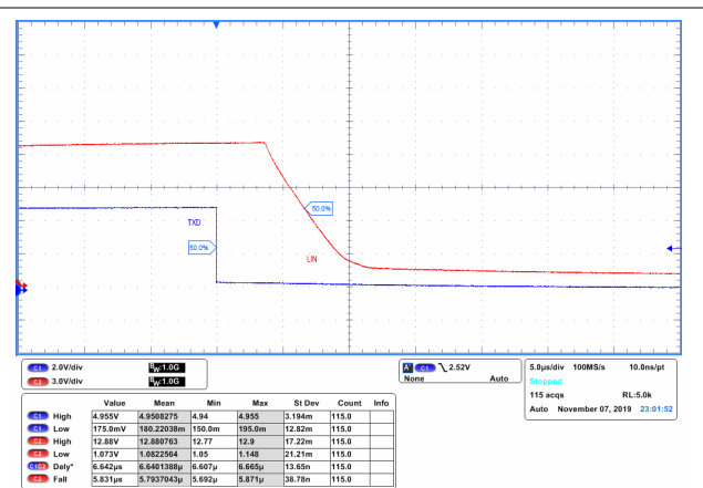
图 10-3. Recessive to Dominant Propagation Delay
