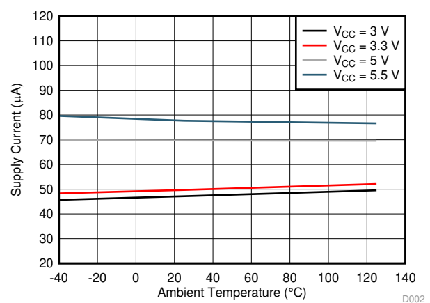
图 4. Supply Current vs Ambient Temperature
