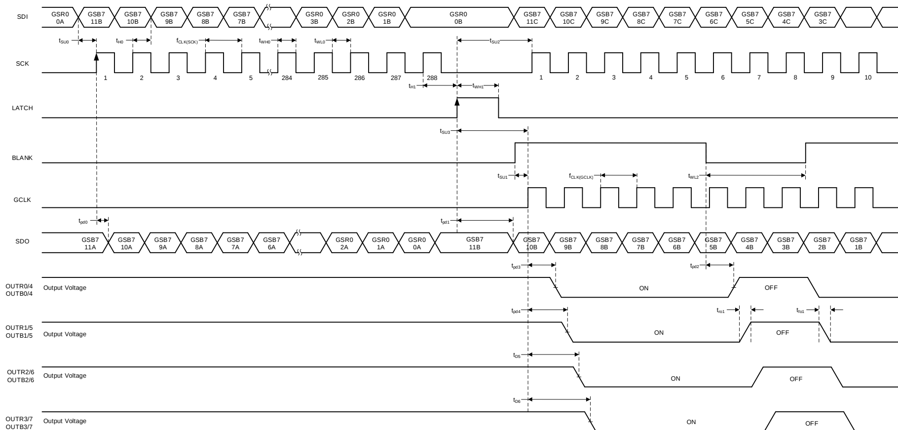
图 1. Grayscale (GS) Data Write
