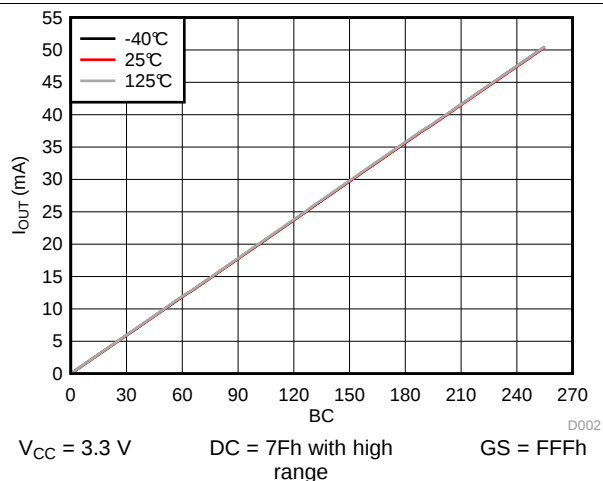
图 20. I_{OUT} vs Brightness Control at Different Ambient Temperatures
