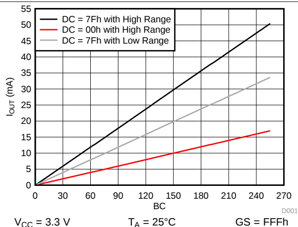
图 19. I_{OUT} vs Brightness Control in Different DC Range
