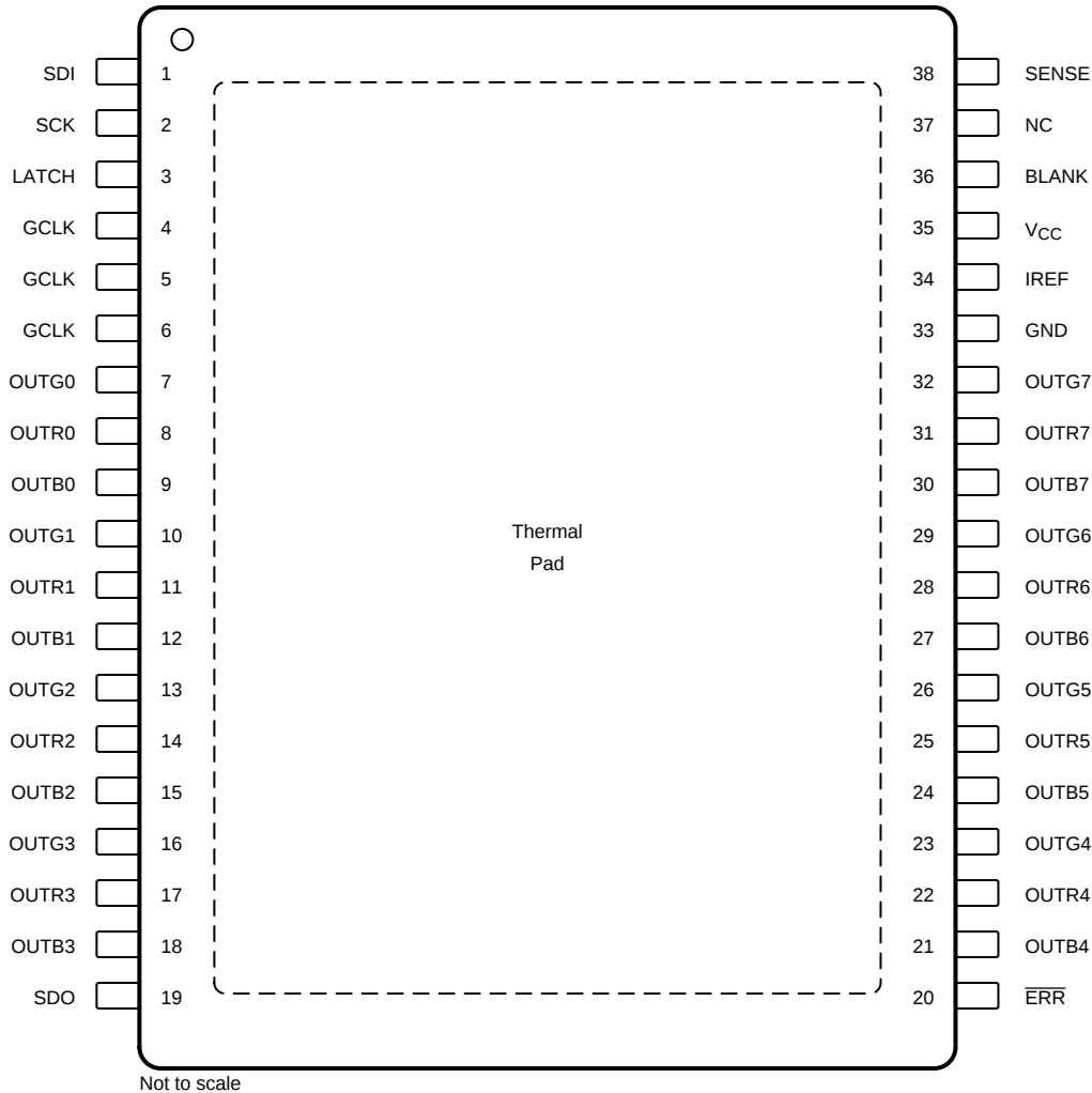
Pin Functions
